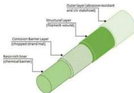
TYPICAL CONSTRUCTION OF FILAMENT WOUND RTR PIPE
