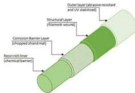
TYPICAL CONSTRUCTION OF FILAMENT WOUND RTR PIPE
